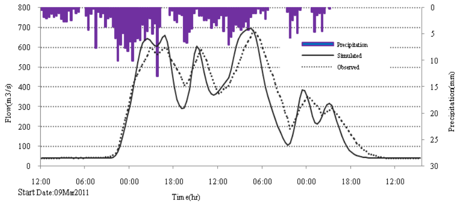
Fig 6. Observed vs. simulated flow in Mar 2011 for Kabkian basin calibration
