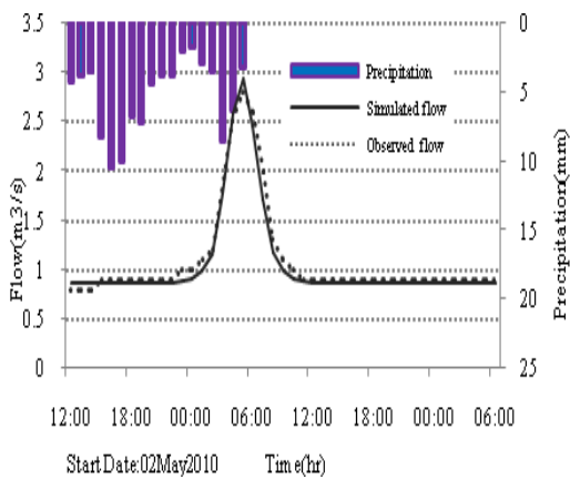
Fig 8. Observed vs. simulated flow in May 2010 for Delibajak basin calibration
