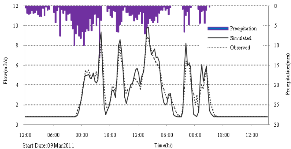
Fig 9. Observed vs. simulated flow in Mar 2011 for Delibajak basin calibration
