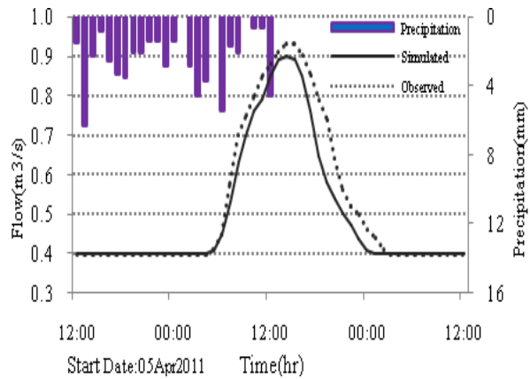
Fig 7. Observed vs. simulated flow in Apr 2011 for Delibajak basin validation
