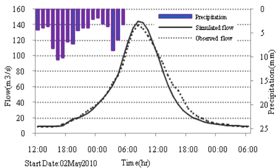
Fig 4. Observed vs. simulated flow in May 2010 for Kabkian basin calibration
