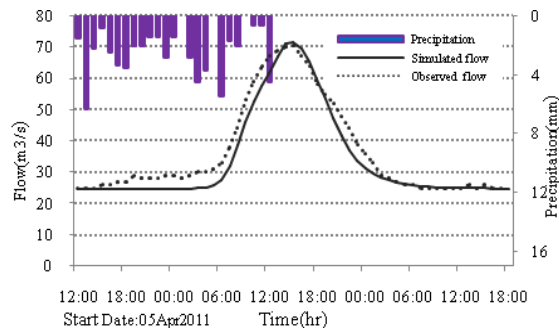
Fig 5. Observed vs. simulated flow in Apr 2011 for Kabkian basin validation
